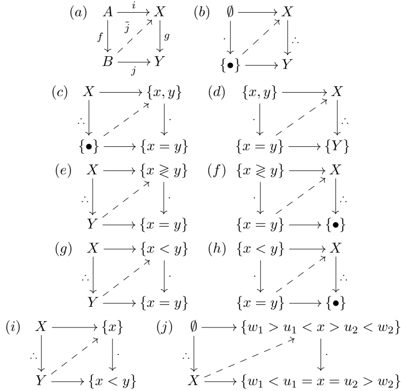
FIGURE 1. The definition and some examples of lifting properties. (a) The definition of a lifting property. (b) X \rightarrow Y is surjective (c) X is connected (d) X \rightarrow Y is injective (e) X \rightarrow Y is injective (f) X satisfies separation axiom T_0 (g) topology on X is the pullback topology via the map X \rightarrow Y (h) X satisfies separation axiom T_1 (i) the image of X is dense in Y (j) X satisfies separation axiom T_4
